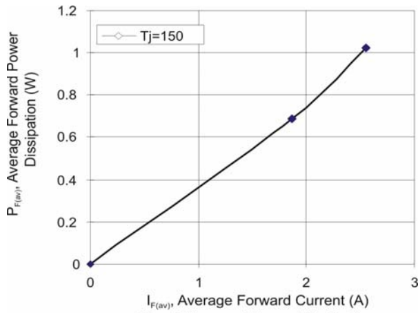
Fig. 5: Forward Power Dissipation
